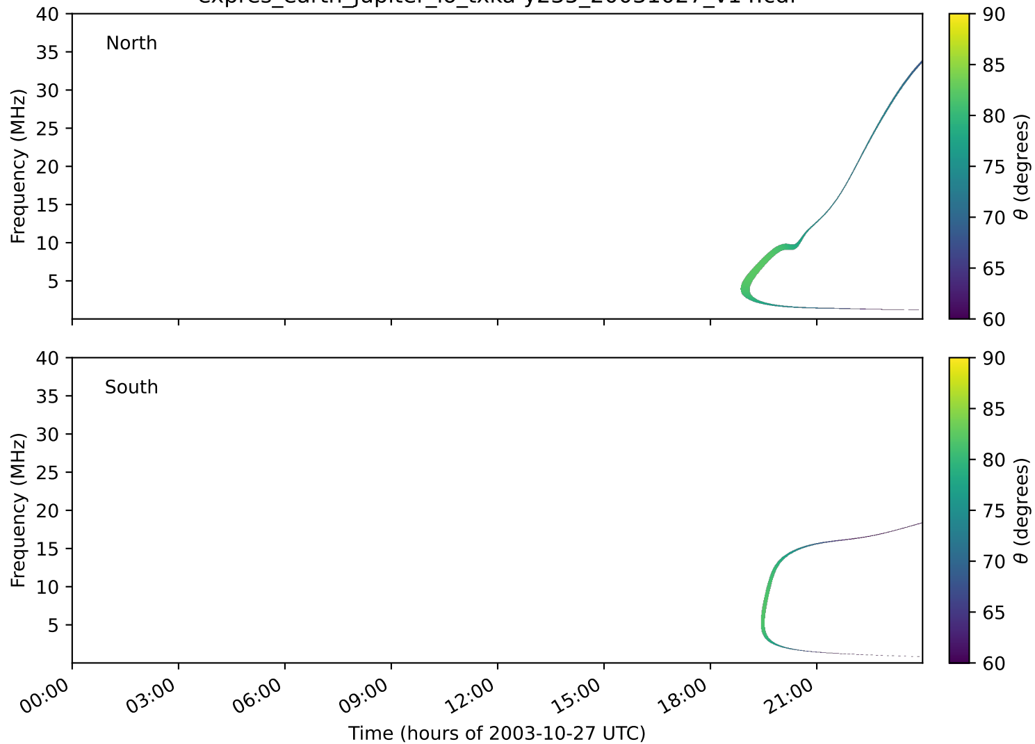
expres_earth_jupiter_io_txka-y235_20031027_v14.cdf
