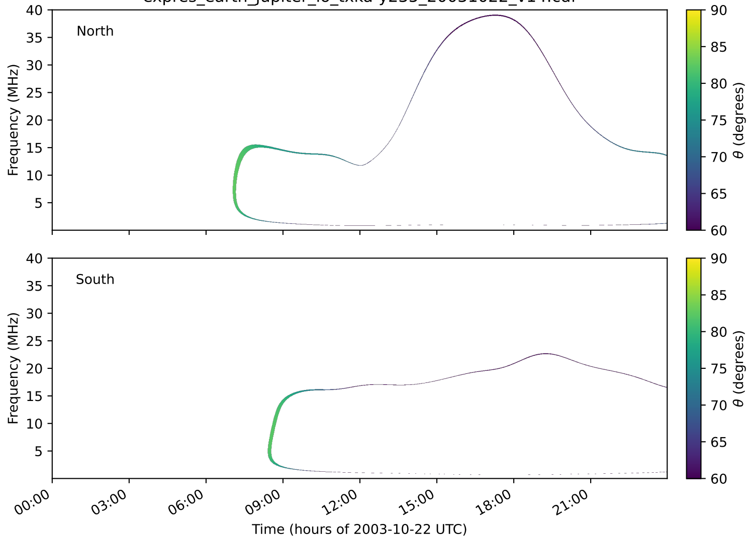
expres_earth_jupiter_io_txka-y235_20031022_v14.cdf
