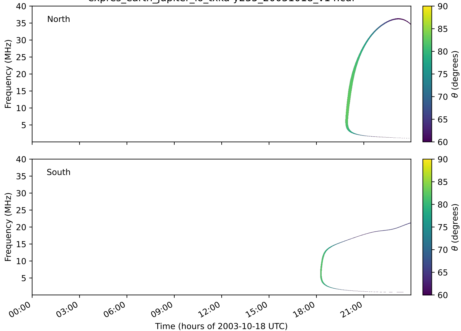
expres_earth_jupiter_io_txka-y235_20031018_v14.cdf
