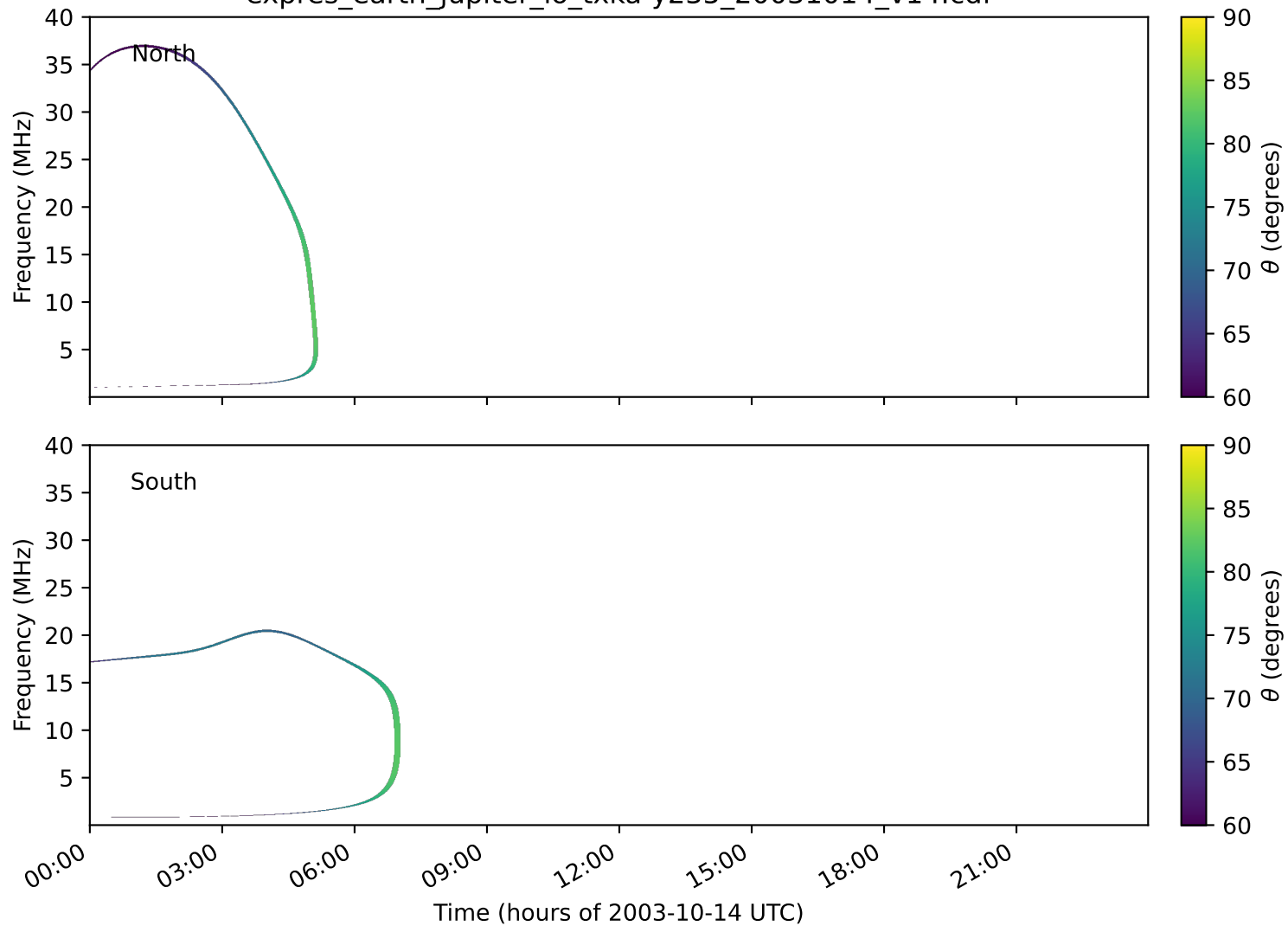
expres_earth_jupiter_io_txka-y235_20031014_v14.cdf
