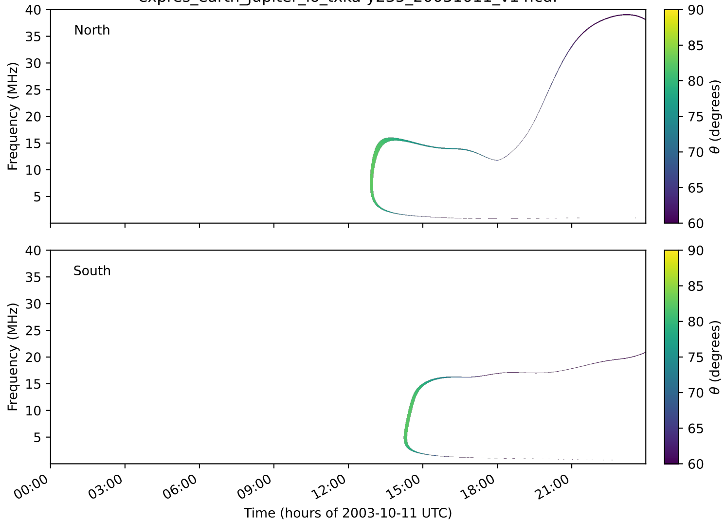
expres_earth_jupiter_io_txka-y235_20031011_v14.cdf
