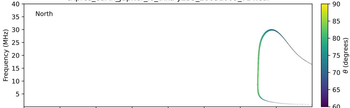
expres_earth_jupiter_io_txka-y235_20031009_v14.cdf
