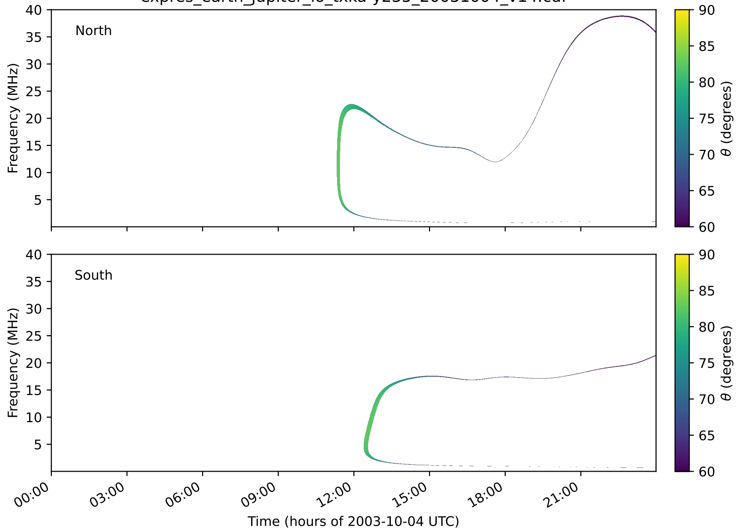
expres_earth_jupiter_io_txka-y235_20031004_v14.cdf
