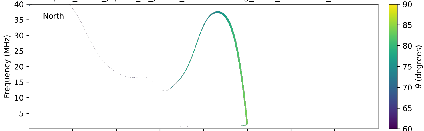
expres_earth_jupiter_io_jrm33_lossc-wid1deg_3kev_20031028_v11.cdf
