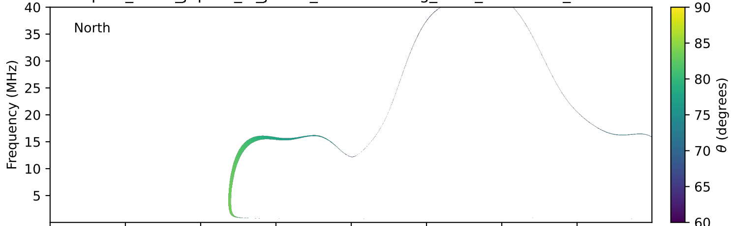
expres_earth_jupiter_io_jrm33_lossc-wid1deg_3kev_20031022_v11.cdf
