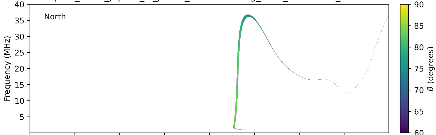
expres_earth_jupiter_io_jrm33_lossc-wid1deg_3kev_20031020_v11.cdf
