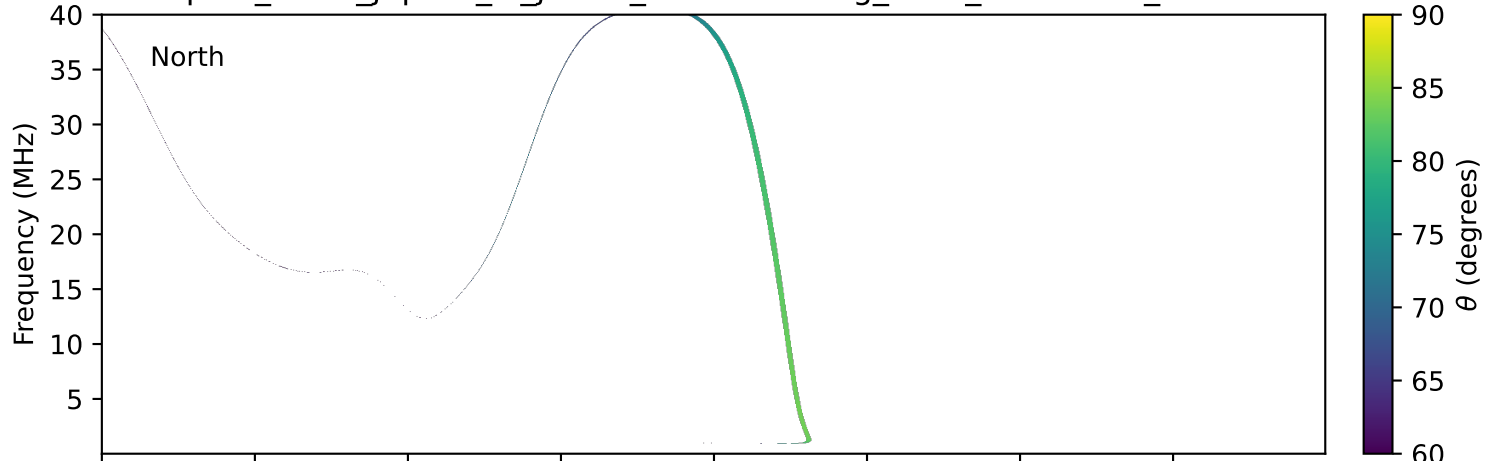
expres_earth_jupiter_io_jrm33_lossc-wid1deg_3kev_20031019_v11.cdf
