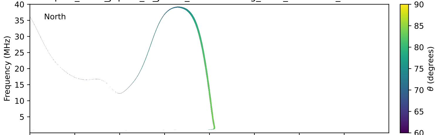
expres_earth_jupiter_io_jrm33_lossc-wid1deg_3kev_20031012_v11.cdf
