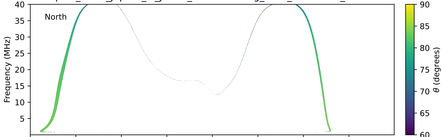
expres_earth_jupiter_io_jrm33_lossc-wid1deg_3kev_20031008_v11.cdf
