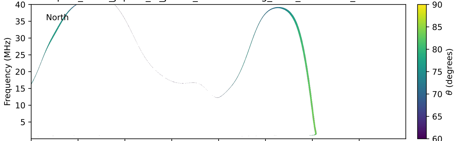
expres_earth_jupiter_io_jrm33_lossc-wid1deg_3kev_20031001_v11.cdf
