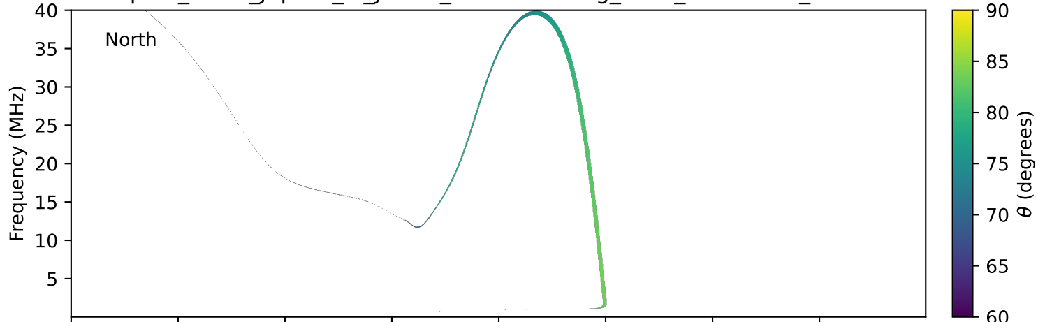
expres_earth_jupiter_io_jrm09_lossc-wid1deg_3kev_20031028_v11.cdf
