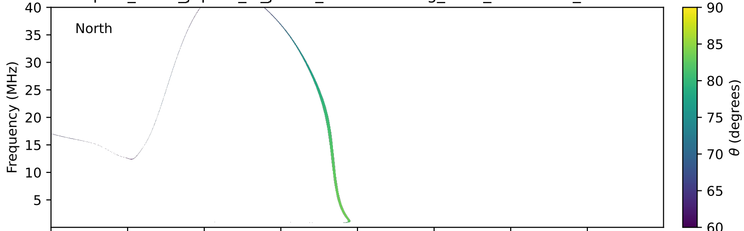
expres_earth_jupiter_io_jrm09_lossc-wid1deg_3kev_20031003_v11.cdf
