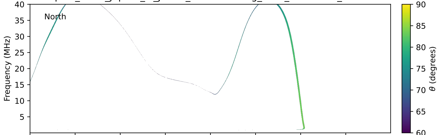
expres_earth_jupiter_io_jrm09_lossc-wid1deg_3kev_20031001_v11.cdf
