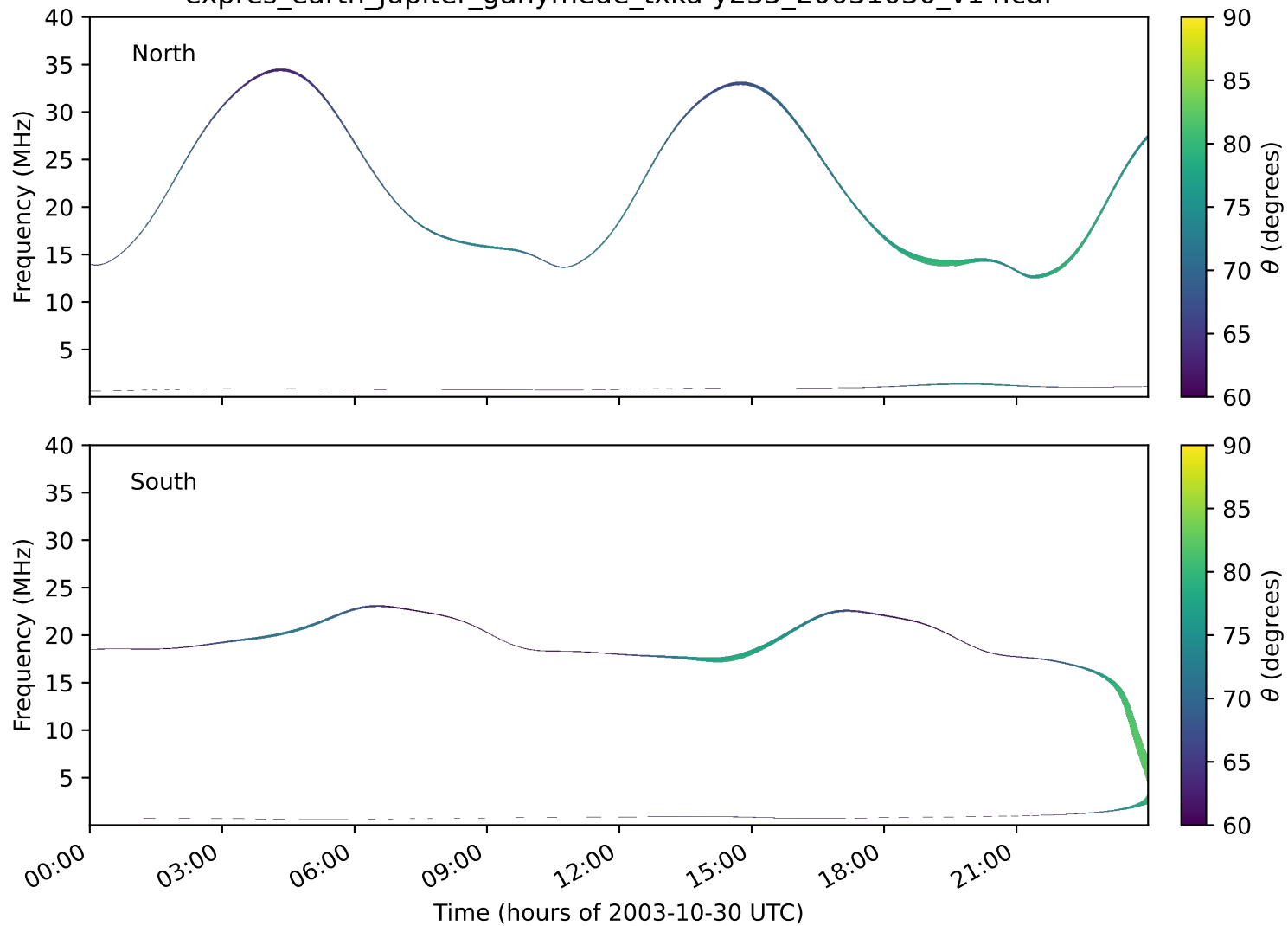
expres_earth_jupiter_ganymede_txka-y235_20031030_v14.cdf
