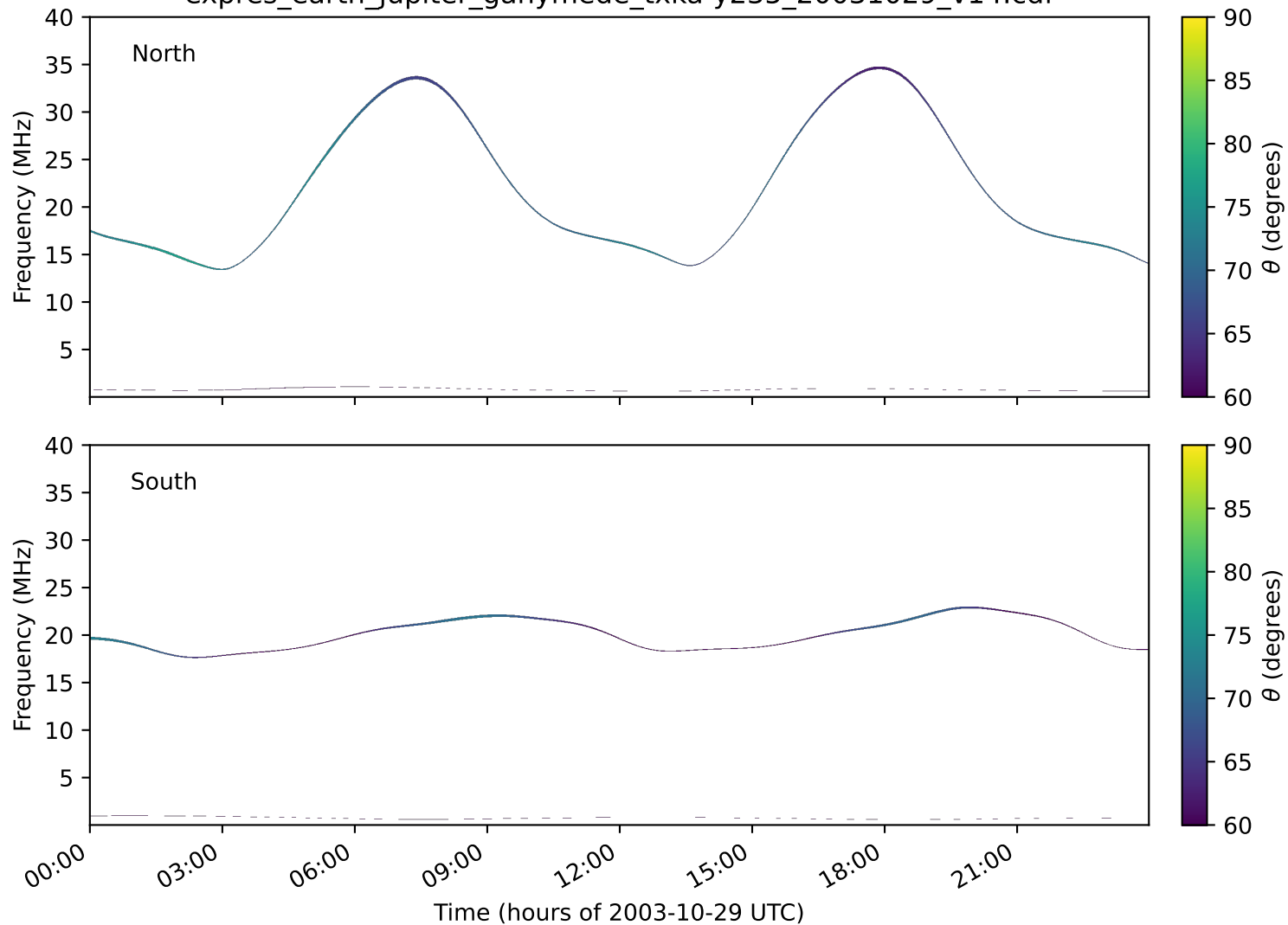
expres_earth_jupiter_ganymede_txka-y235_20031029_v14.cdf
