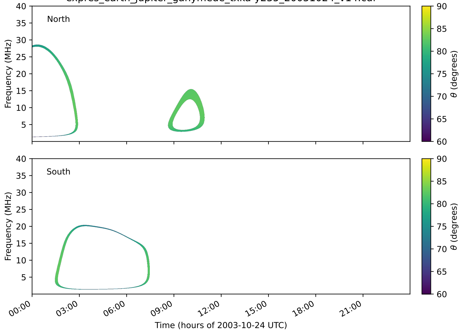
expres_earth_jupiter_ganymede_txka-y235_20031024_v14.cdf
