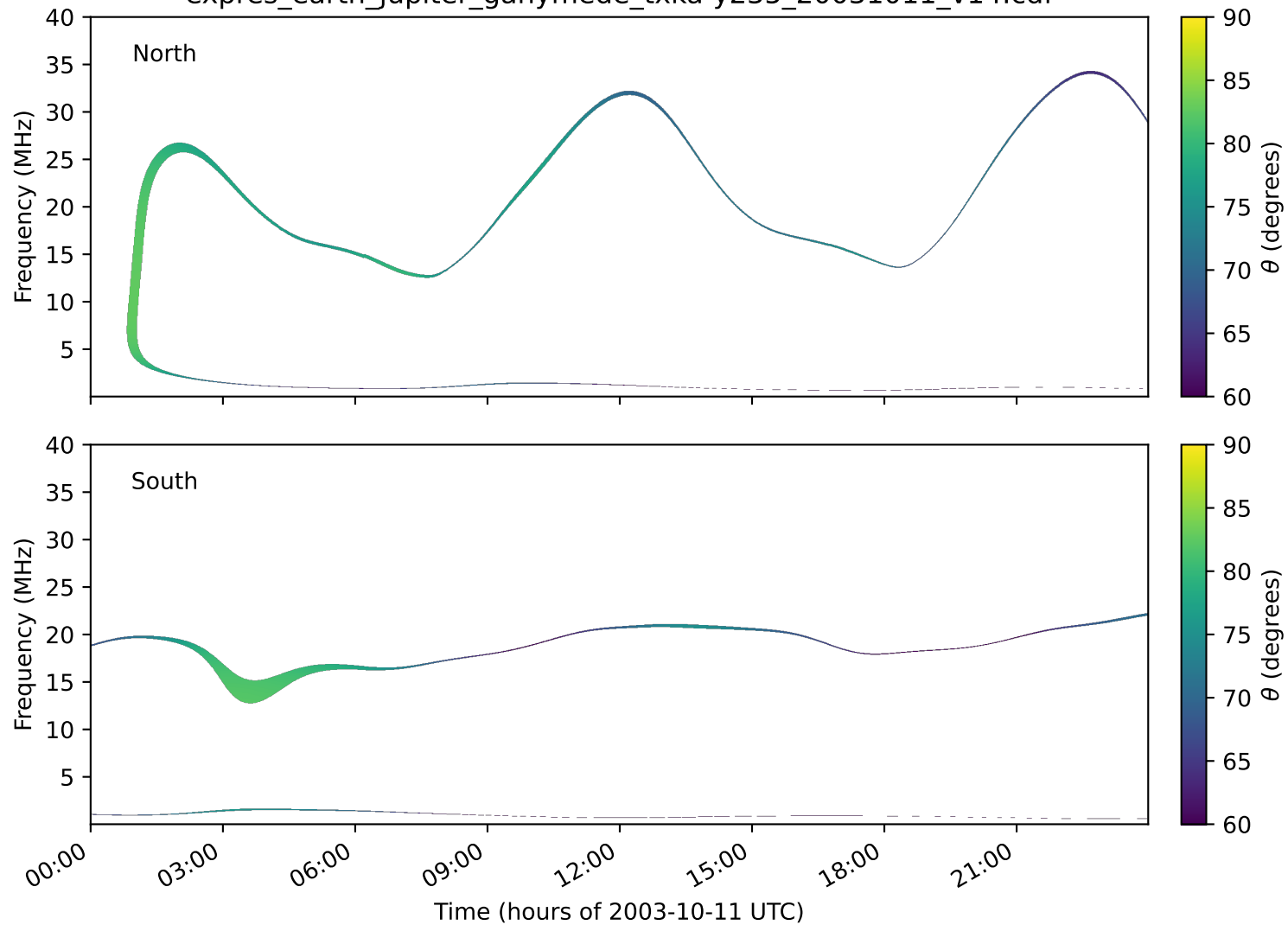
expres_earth_jupiter_ganymede_txka-y235_20031011_v14.cdf
