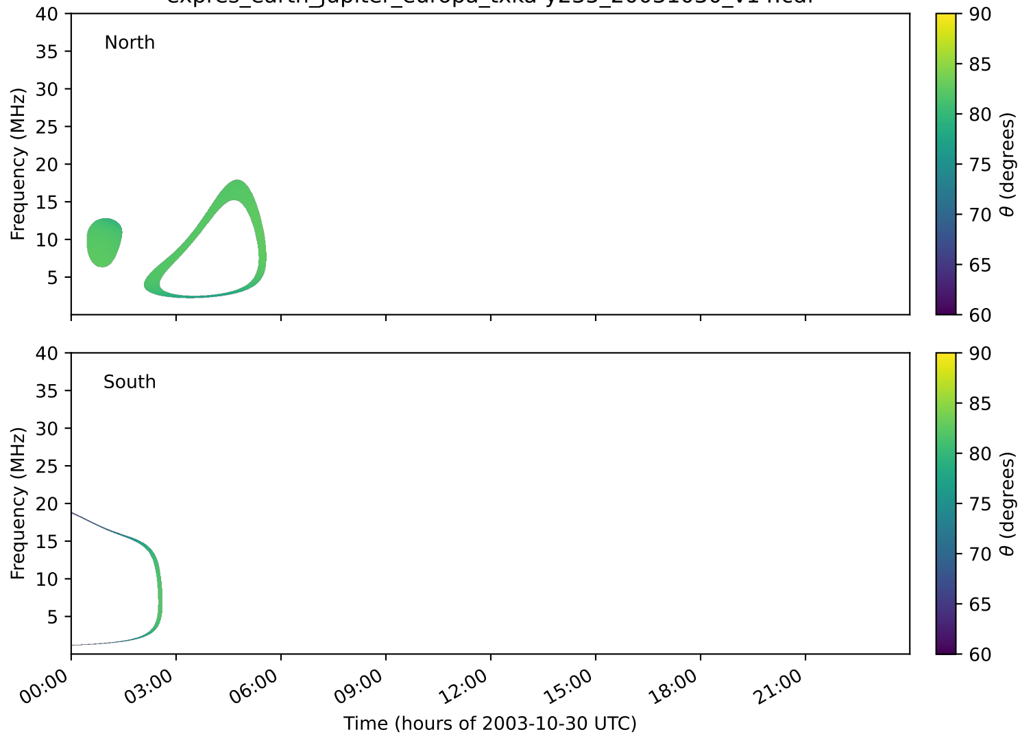
expres_earth_jupiter_europa_txka-y235_20031030_v14.cdf
