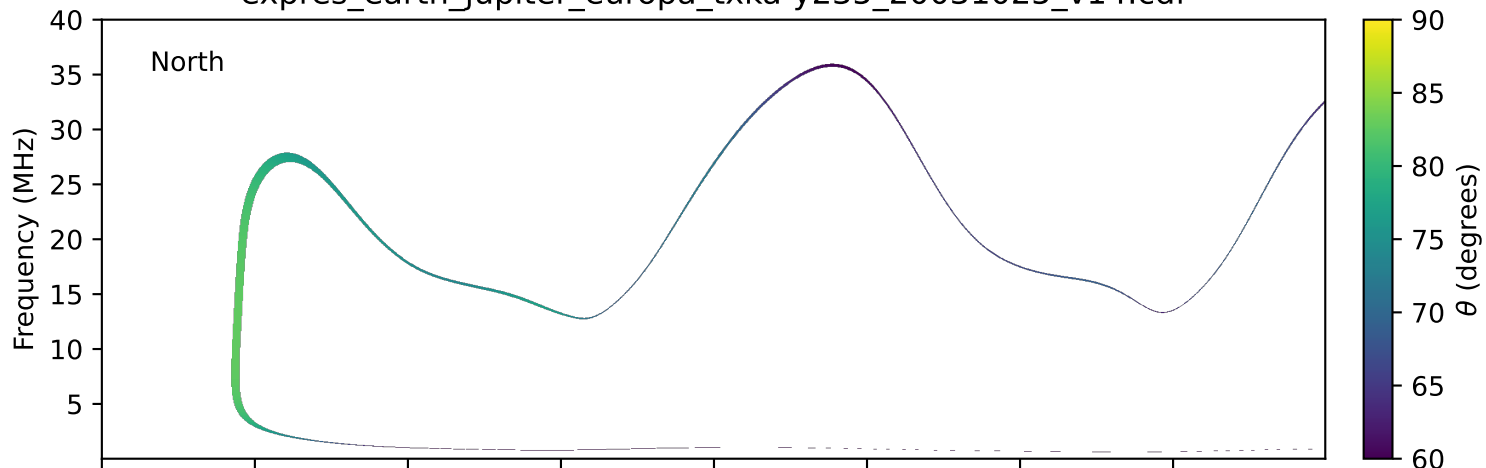
expres_earth_jupiter_europa_txka-y235_20031025_v14.cdf
