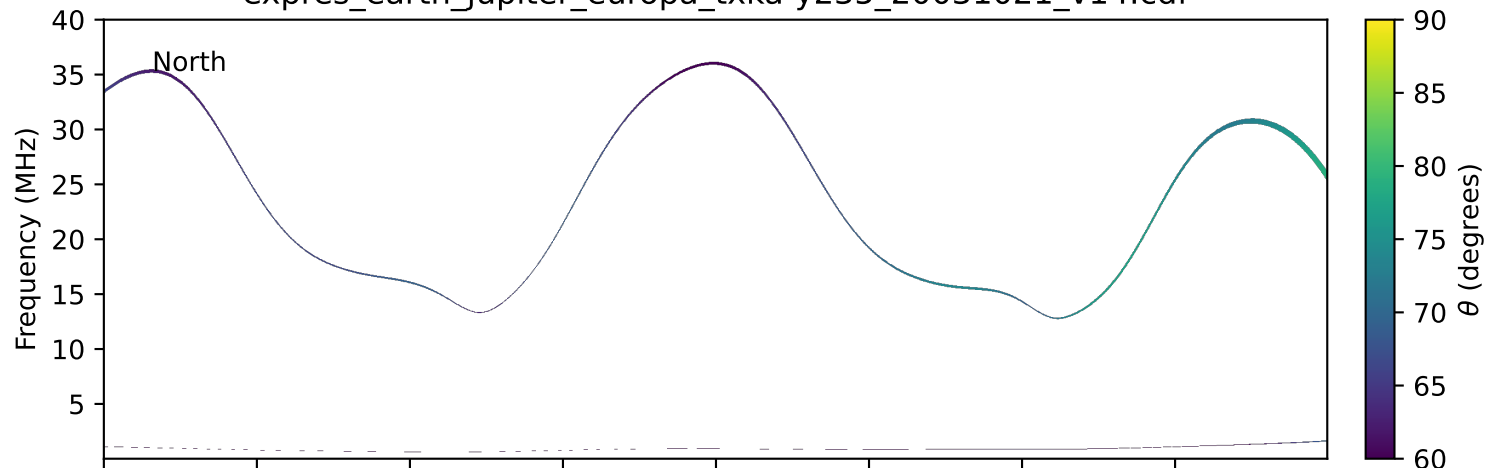
expres_earth_jupiter_europa_txka-y235_20031021_v14.cdf
