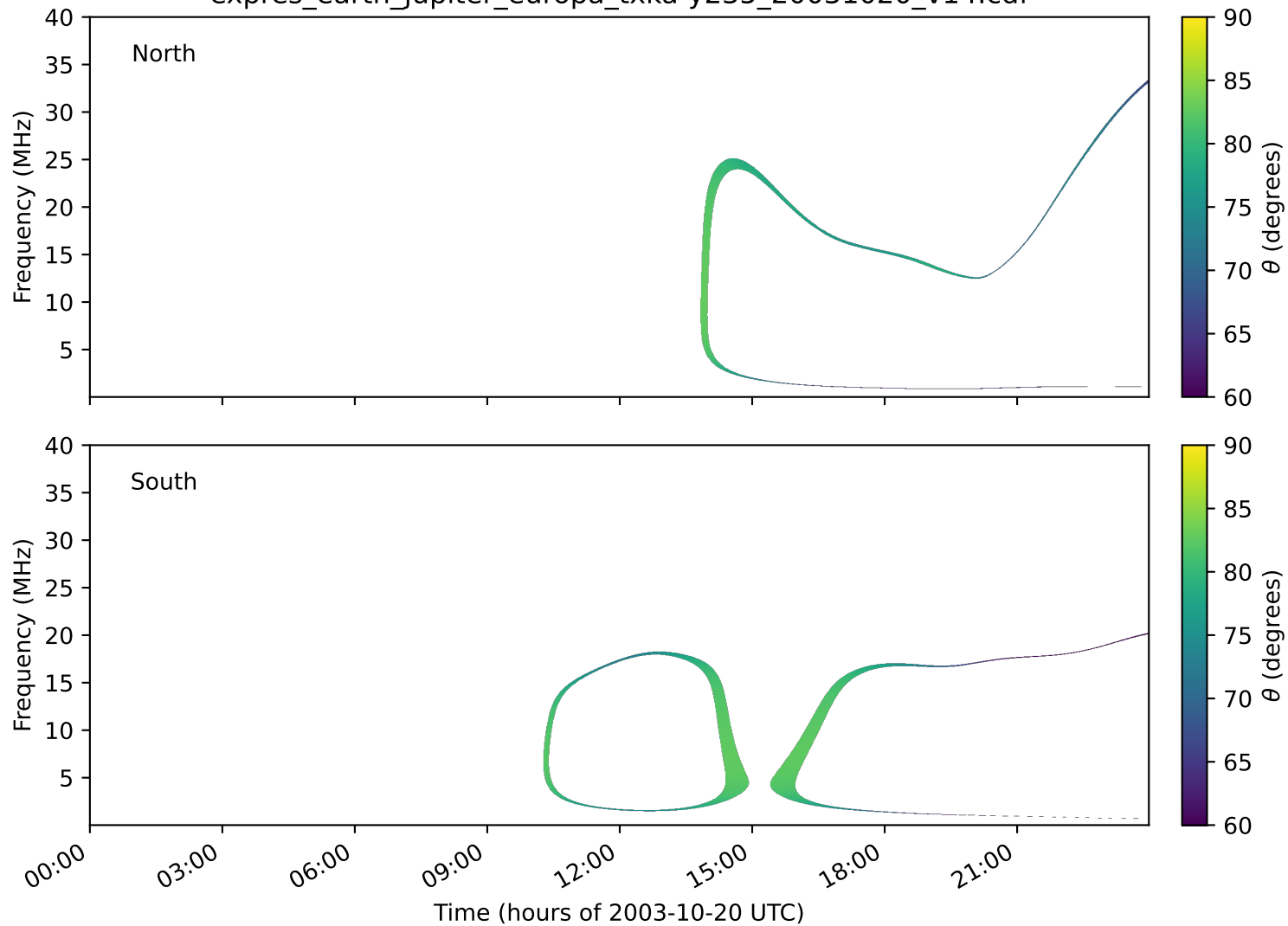
expres_earth_jupiter_europa_txka-y235_20031020_v14.cdf
