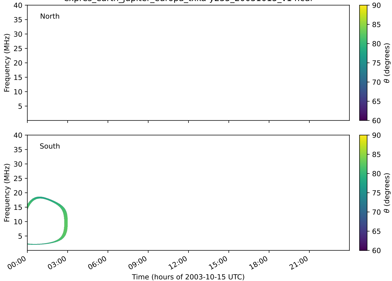
expres_earth_jupiter_europa_txka-y235_20031015_v14.cdf
