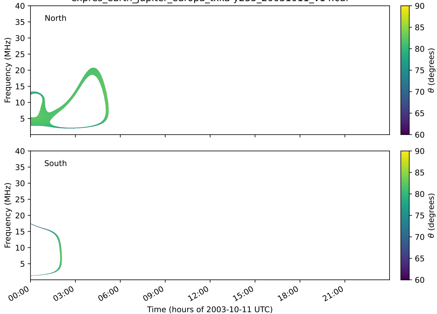
expres_earth_jupiter_europa_txka-y235_20031011_v14.cdf
