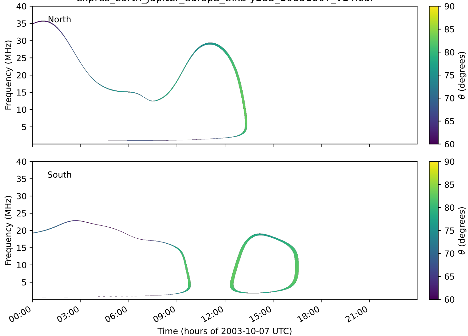
expres_earth_jupiter_europa_txka-y235_20031007_v14.cdf
