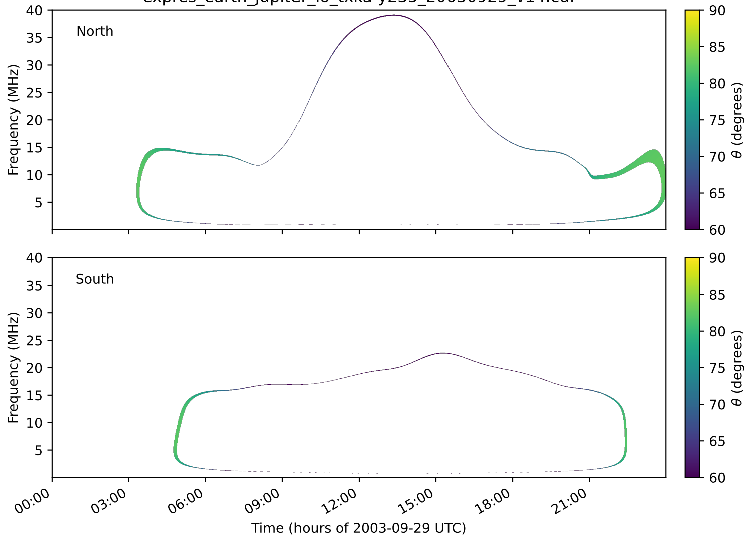
expres_earth_jupiter_io_txka-y235_20030929_v14.cdf
