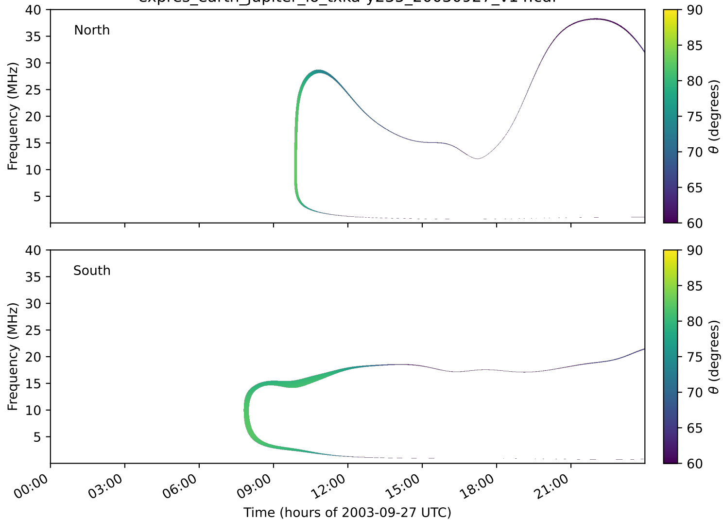
expres_earth_jupiter_io_txka-y235_20030927_v14.cdf
