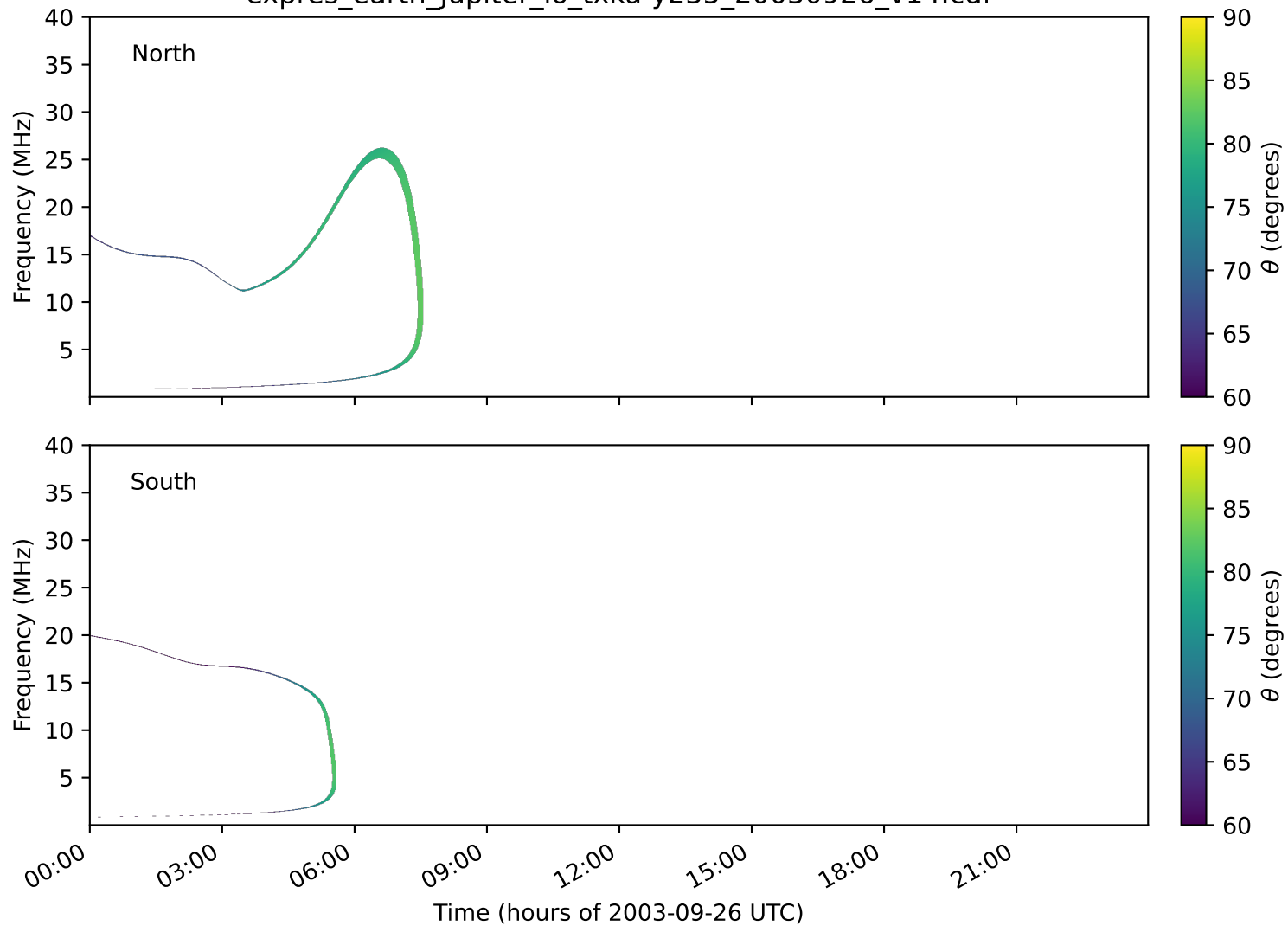
expres_earth_jupiter_io_txka-y235_20030926_v14.cdf
