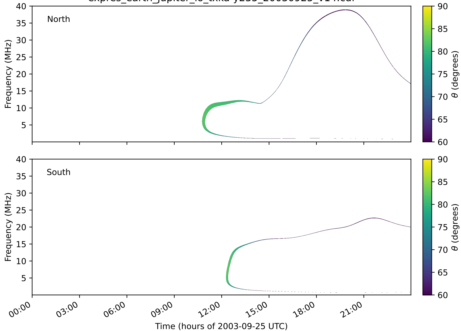
expres_earth_jupiter_io_txka-y235_20030925_v14.cdf
