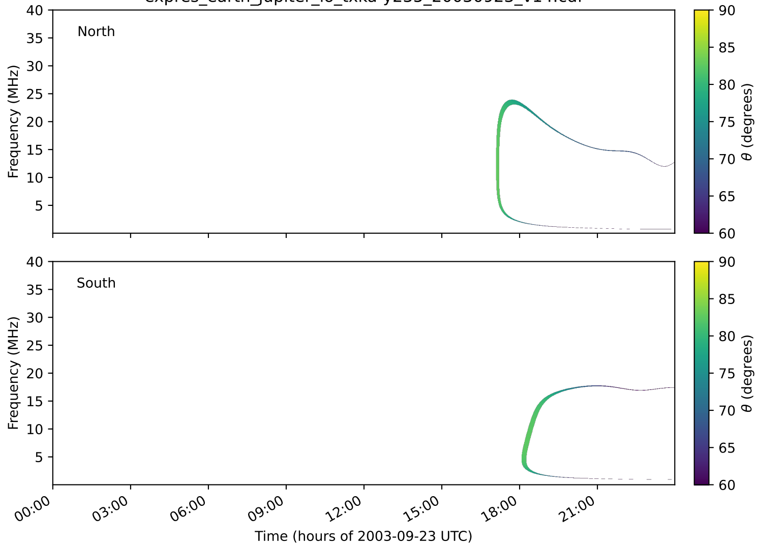
expres_earth_jupiter_io_txka-y235_20030923_v14.cdf
