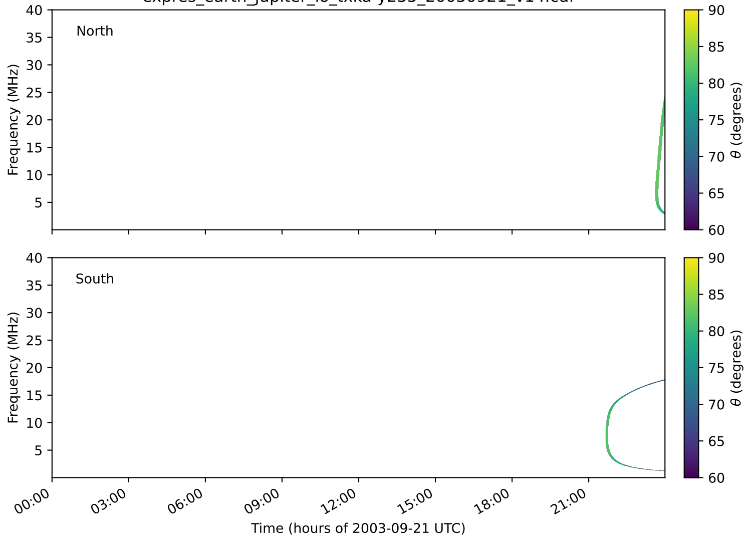
expres_earth_jupiter_io_txka-y235_20030921_v14.cdf
