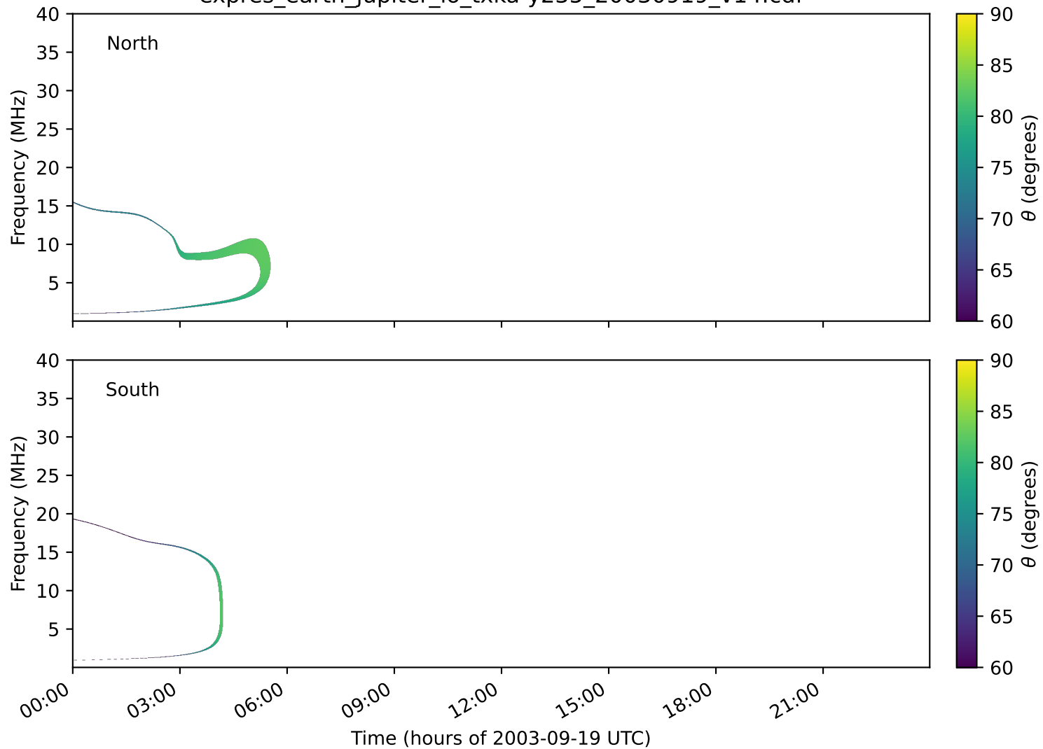
expres_earth_jupiter_io_txka-y235_20030919_v14.cdf
