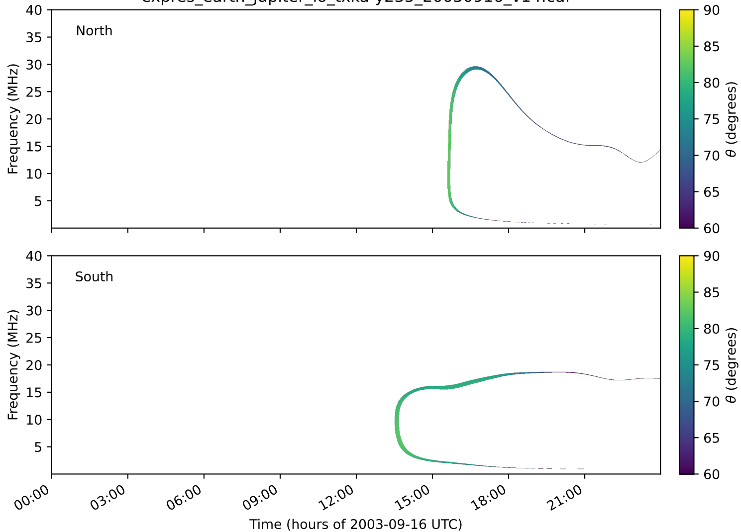
expres_earth_jupiter_io_txka-y235_20030916_v14.cdf
