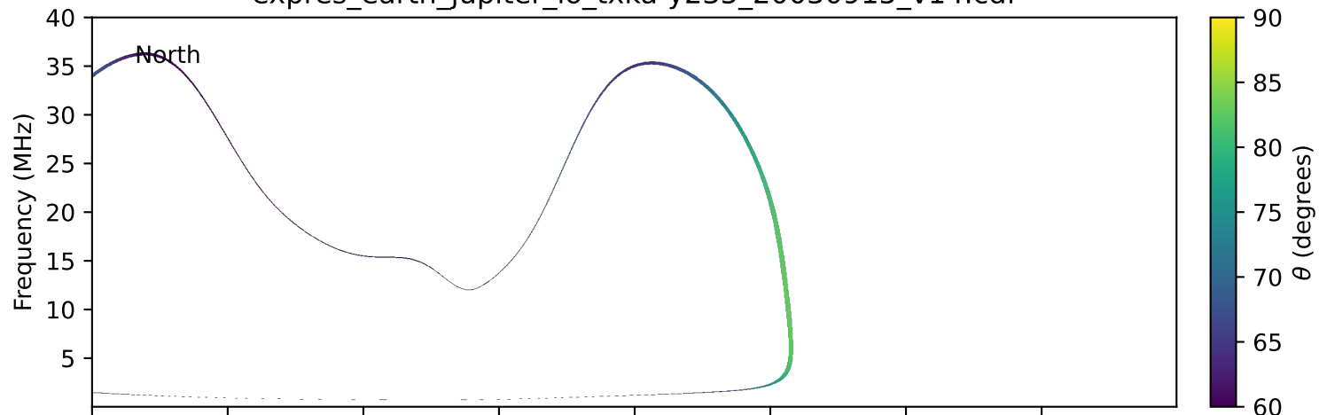
expres_earth_jupiter_io_txka-y235_20030915_v14.cdf
