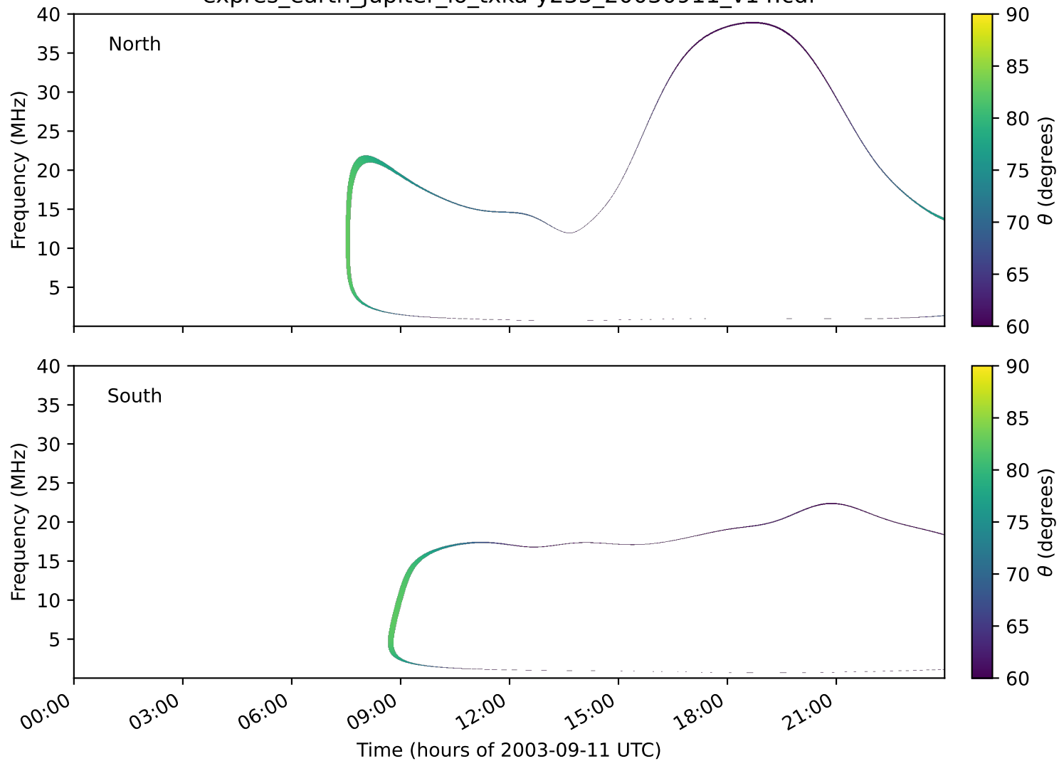
expres_earth_jupiter_io_txka-y235_20030911_v14.cdf
