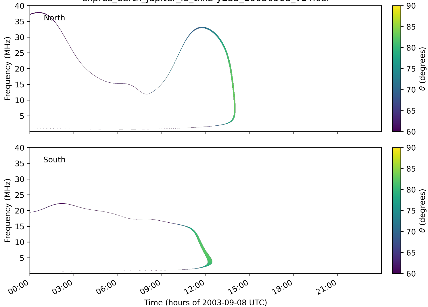
expres_earth_jupiter_io_txka-y235_20030908_v14.cdf
