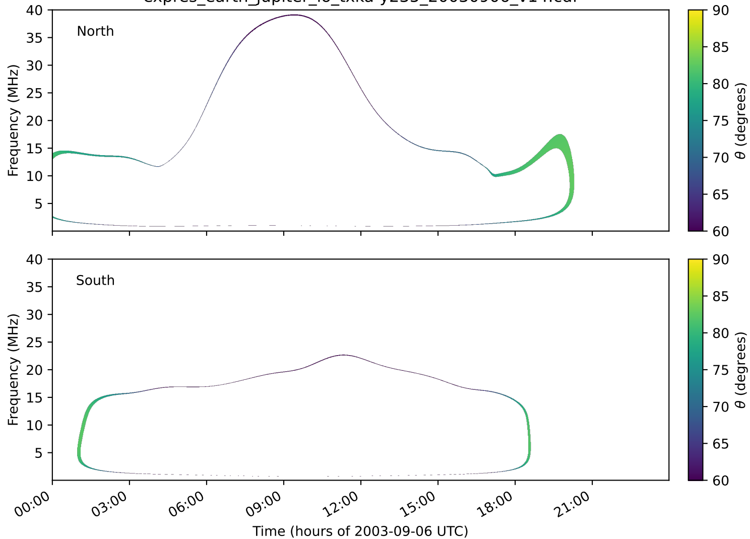
expres_earth_jupiter_io_txka-y235_20030906_v14.cdf
