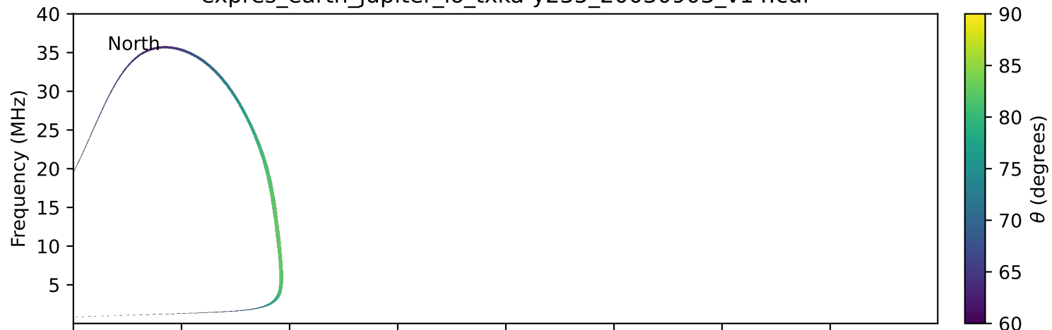
expres_earth_jupiter_io_txka-y235_20030903_v14.cdf
