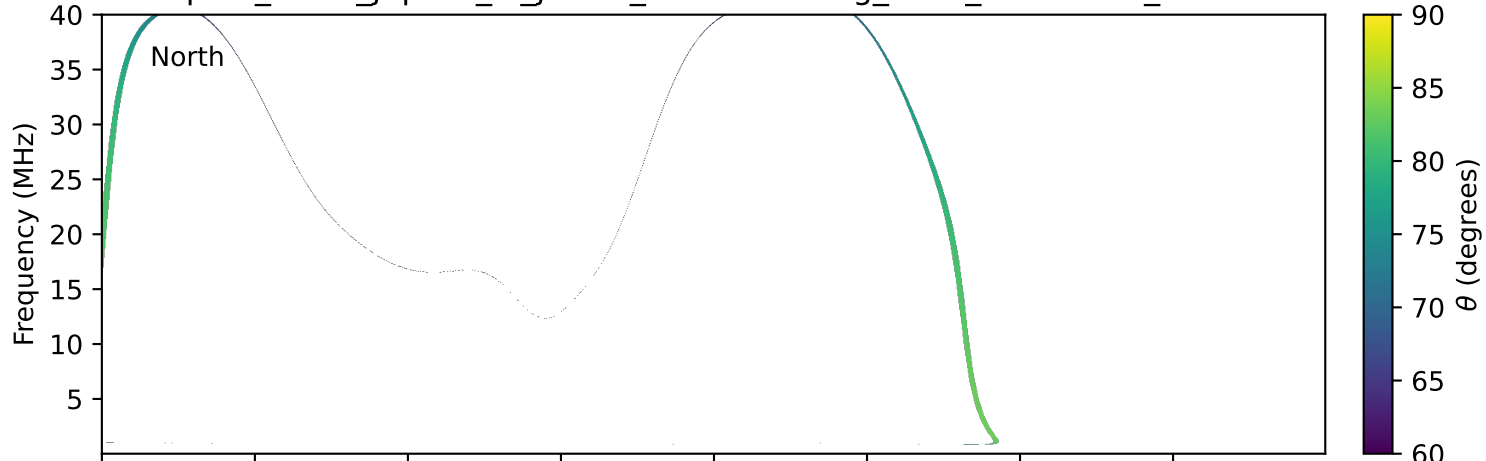
expres_earth_jupiter_io_jrm33_lossc-wid1deg_3kev_20030922_v11.cdf
