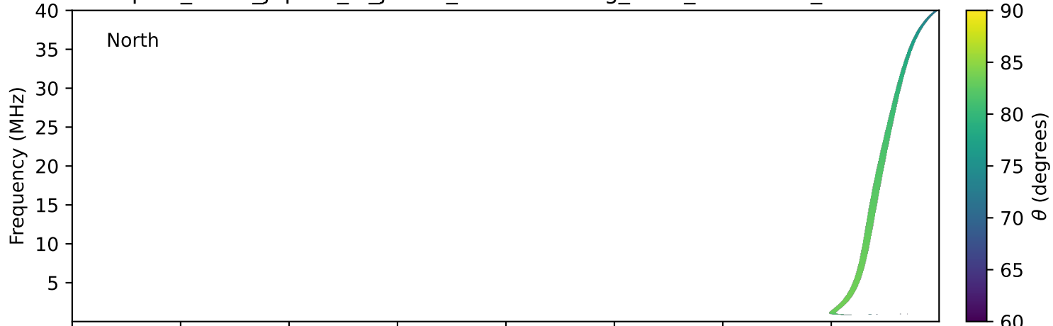
expres_earth_jupiter_io_jrm33_lossc-wid1deg_3kev_20030914_v11.cdf
