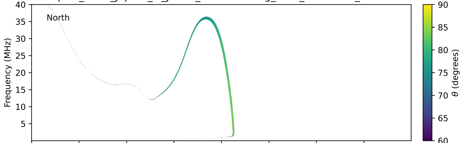
expres_earth_jupiter_io_jrm33_lossc-wid1deg_3kev_20030901_v11.cdf
