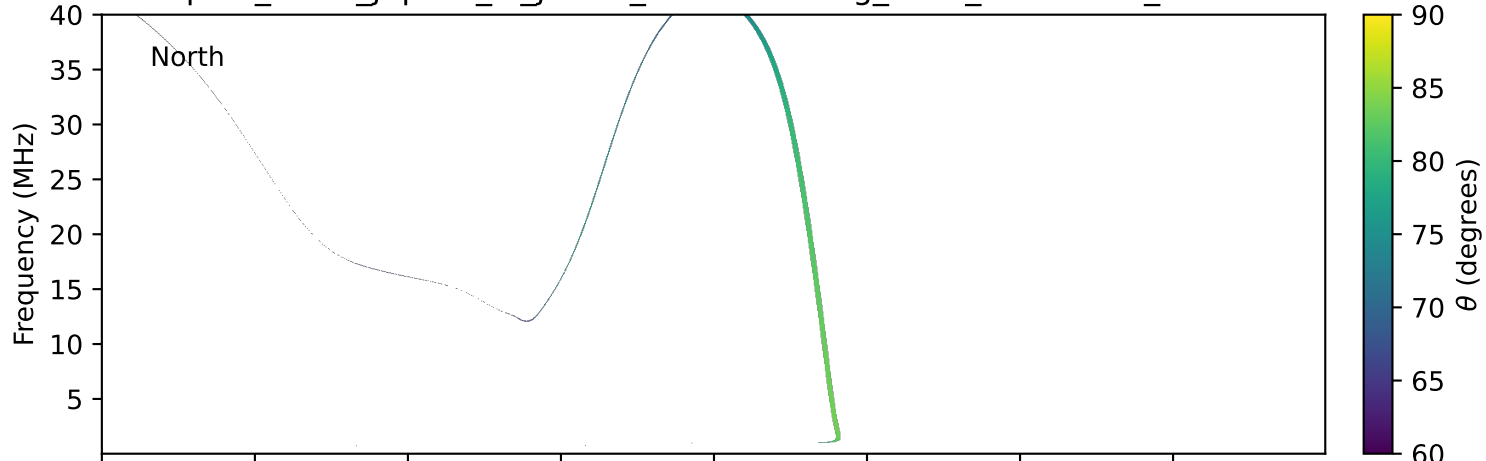
expres_earth_jupiter_io_jrm09_lossc-wid1deg_3kev_20030908_v11.cdf
