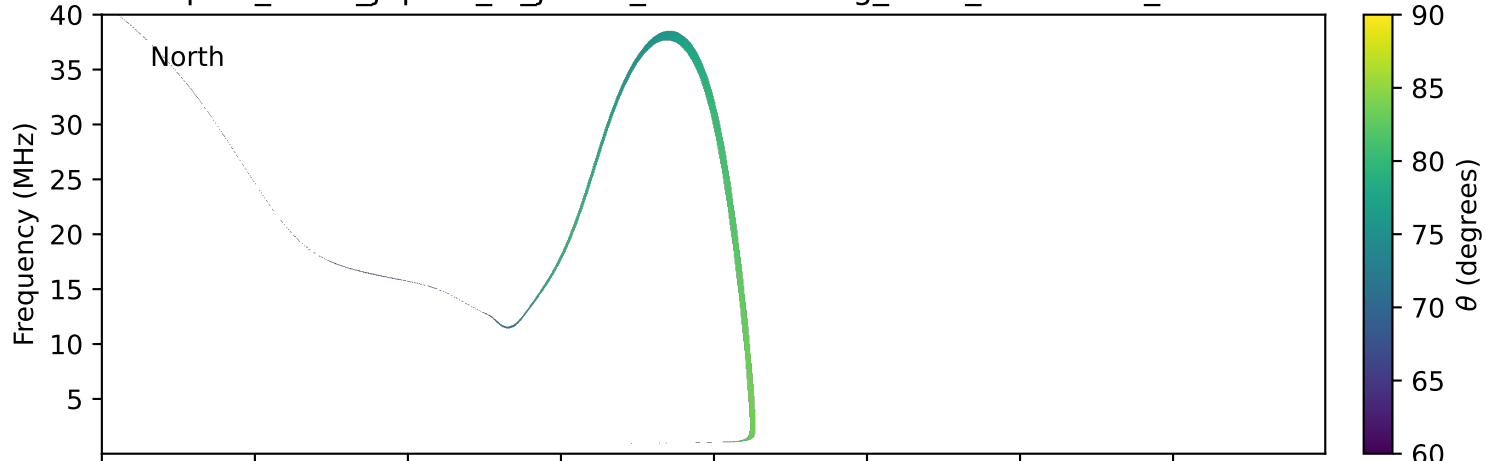
expres_earth_jupiter_io_jrm09_lossc-wid1deg_3kev_20030901_v11.cdf
