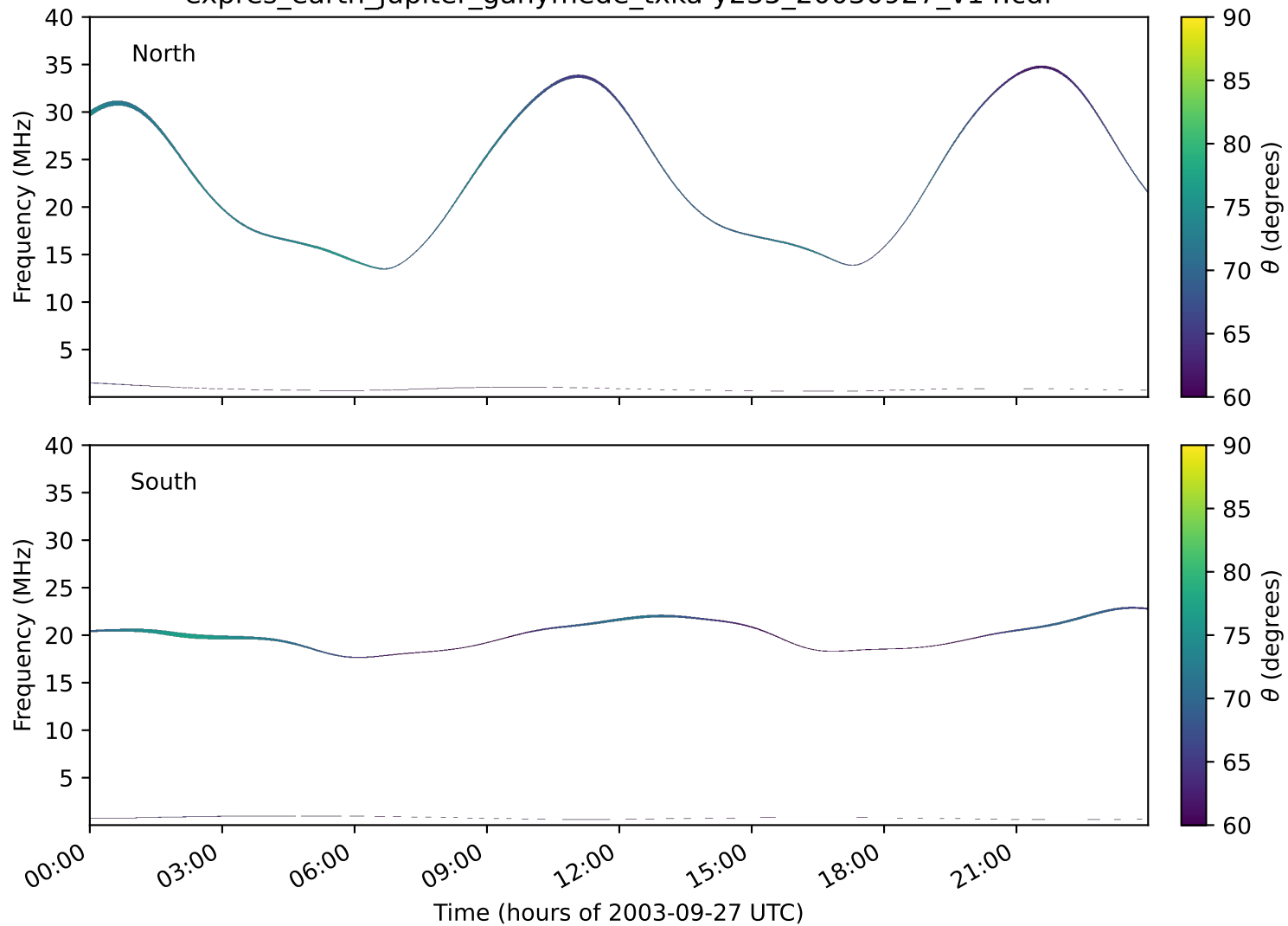
expres_earth_jupiter_ganymede_txka-y235_20030927_v14.cdf
