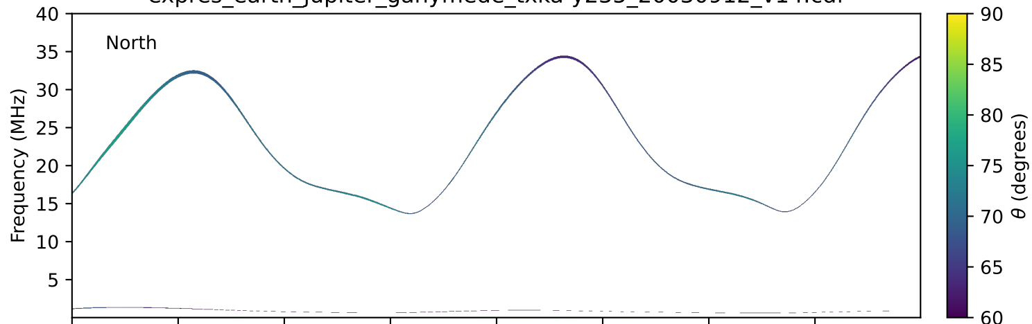
expres_earth_jupiter_ganymede_txka-y235_20030912_v14.cdf
