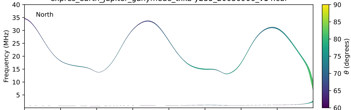
expres_earth_jupiter_ganymede_txka-y235_20030906_v14.cdf
