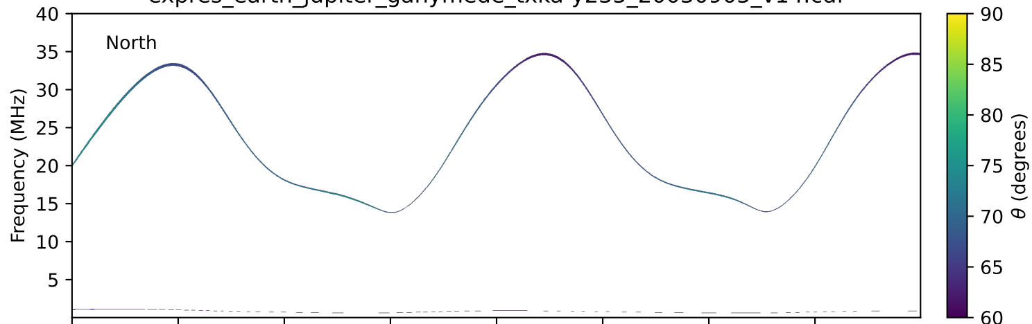
expres_earth_jupiter_ganymede_txka-y235_20030905_v14.cdf
